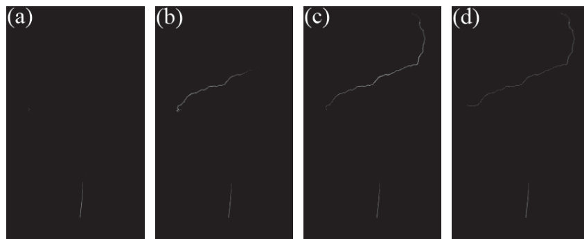
Fig. 1 Distributions of simulated total charge density in different time: (a) 20th minute, (b) 30th minute, (c) 60th minute, (d) 90th minute. The contour lines are isotherms (unit: ^{\circ}\text{C} ).
