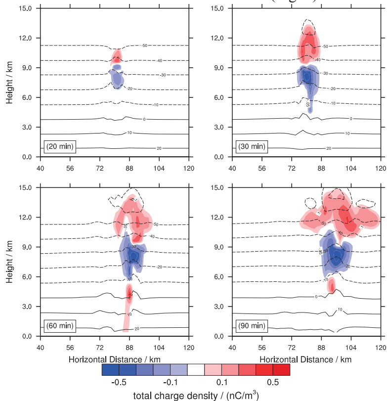
Fig. 1 Distributions of simulated total charge density in different time: (a) 20th minute, (b) 30th minute, (c) 60th minute, (d) 90th minute. The contour lines are isotherms (unit: ^{\circ}\text{C} ).
